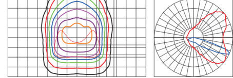
T4S Type IV Short
