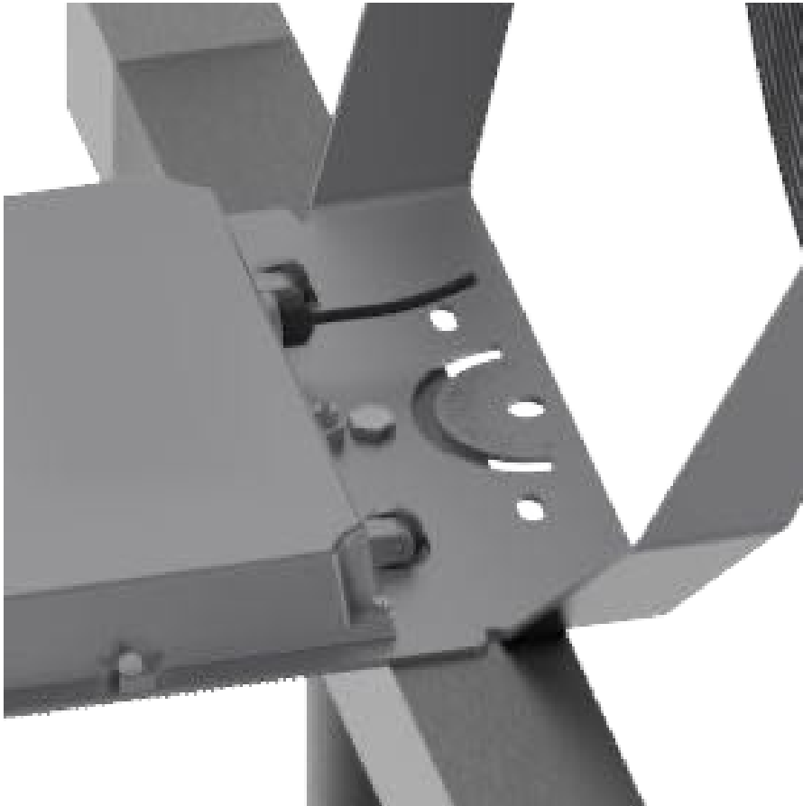
U-Bracket Mount
